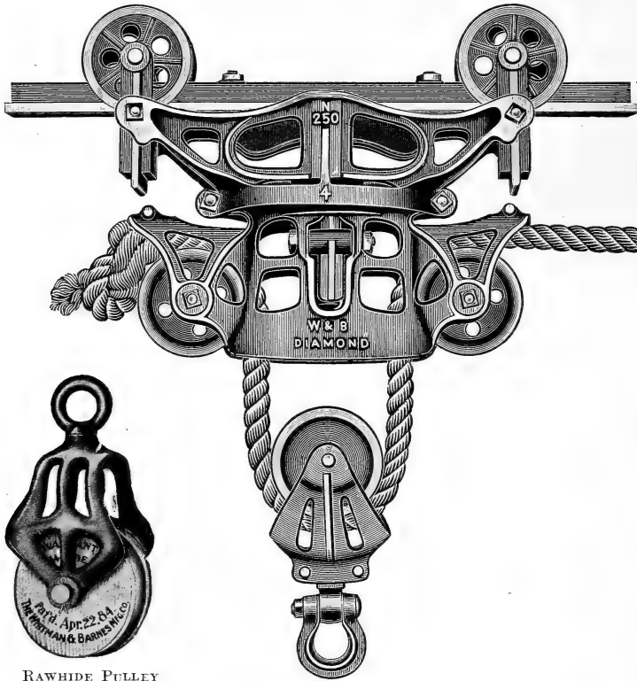
RAWHIDE PULLEY
